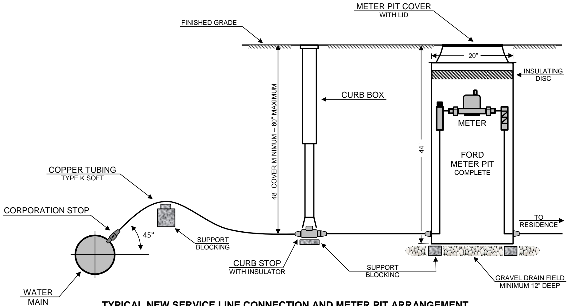
TYPICAL NEW SERVICE LINE CONNECTION AND METER PIT ARRANGEMENT
